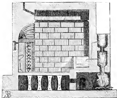
Fig. 393. Hypocaust of a Roman villa at Tusculum.
